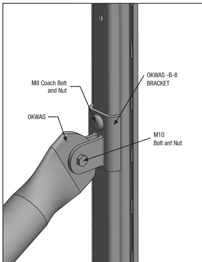
OKWAS Angle Stay
