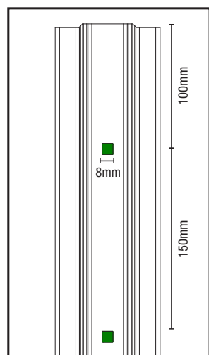
Barb wire slots
