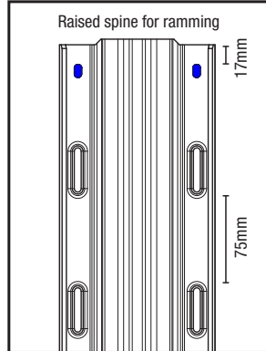
Wire slots
